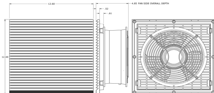
PFFP-500 / 850 CFM
