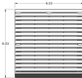
PFFP-100 / 131 CFM
