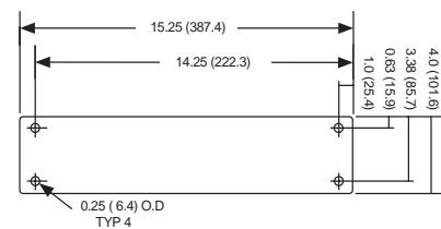
WPS/WPSA Horizontal Mount Flange Front View
