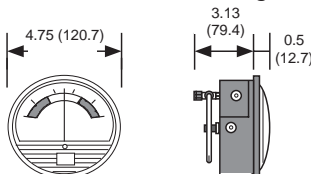
Panel Cutout 4.5 (114.3) Ø
