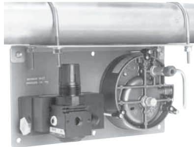
Model 3004-LPS-CI-YZ-HMB Flange Mounted to Horizontal 2" Pipe Stand with Model PMK-1 Fastener Kit
