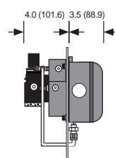
WPS/WPSA (With Pressure Switch)
