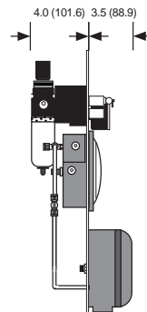
WPS/WPSA (With Pressure Switch)
