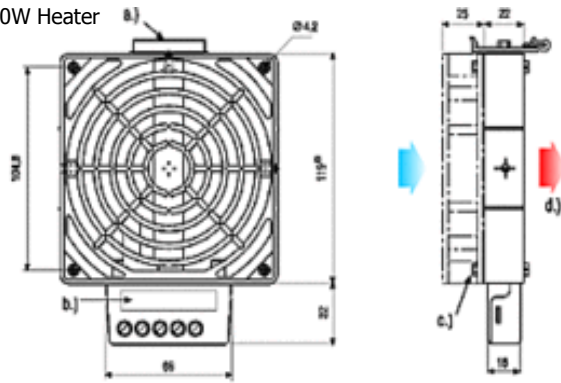
200W/300W/400W Heater
