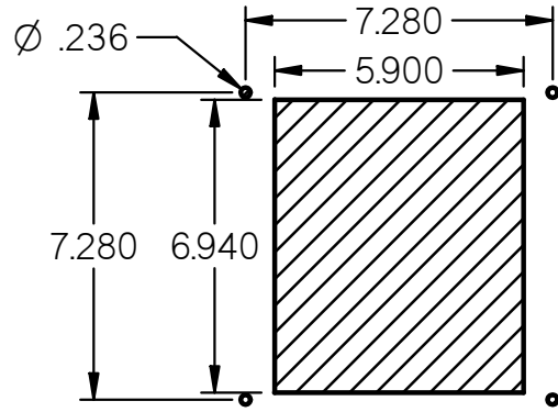
CUTOUT DRAWING 1:5
