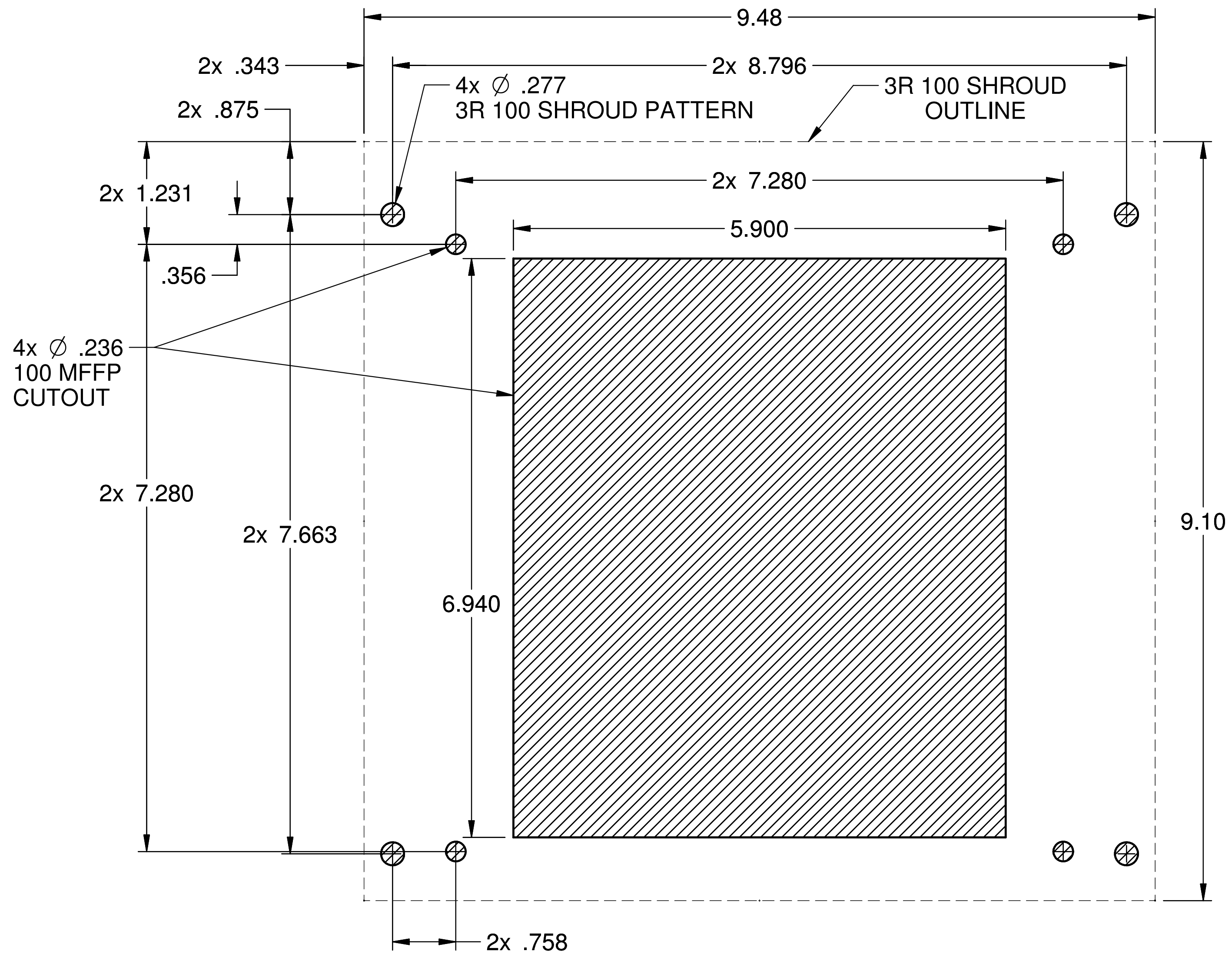
CUTOUT TEMPLATE 100 MFFP WITH 3R 100 RAIN SHROUD (VERIFY PRINT ACCURACY BEFORE USE)
