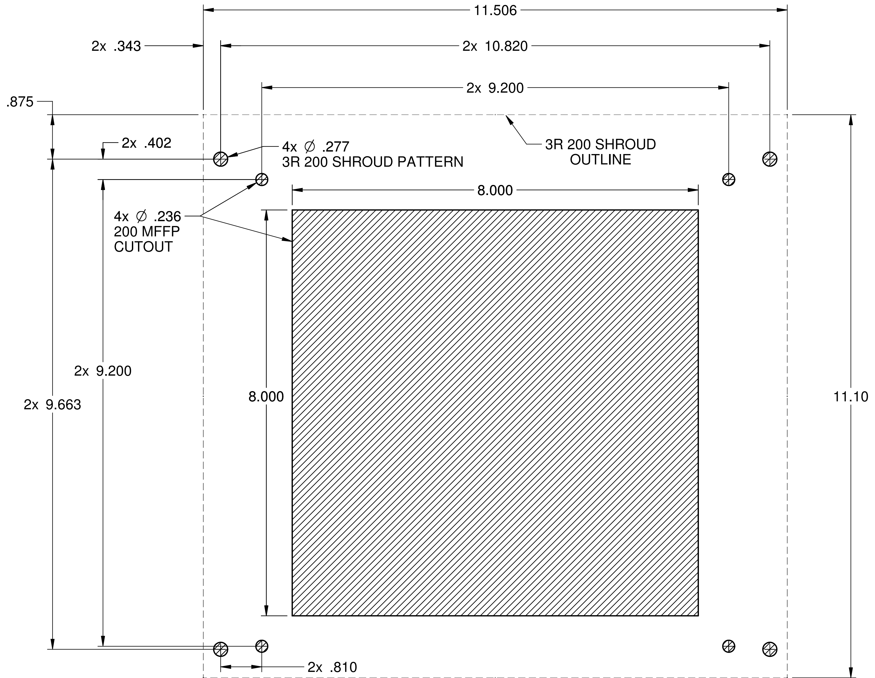
CUTOUT TEMPLATE 200 MFFP WITH 3R 200 RAIN SHROUD (VERIFY PRINT ACCURACY BEFORE USE)
