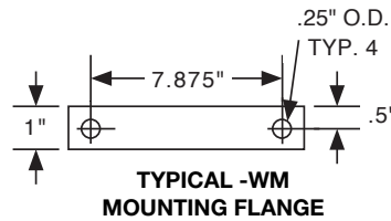
1001B-LPS-WM (Wall Mount Configuration)
