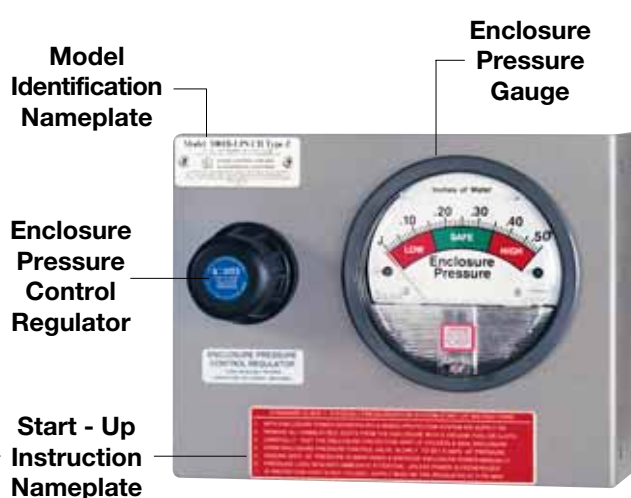
Model 1001B-LPS Front View
