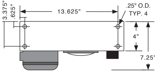
1001B-WPS-BM (Bottom Mount Configuration)
