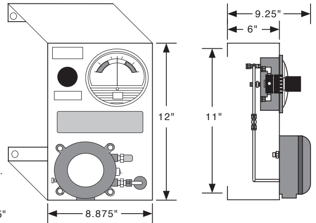
1001B-WPS-WM (Wall Mount Configuration)
