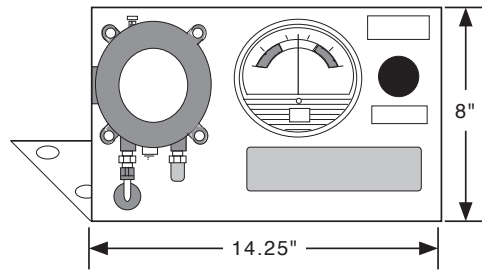
1001B-LPS-RH (Right Hand Configuration)
