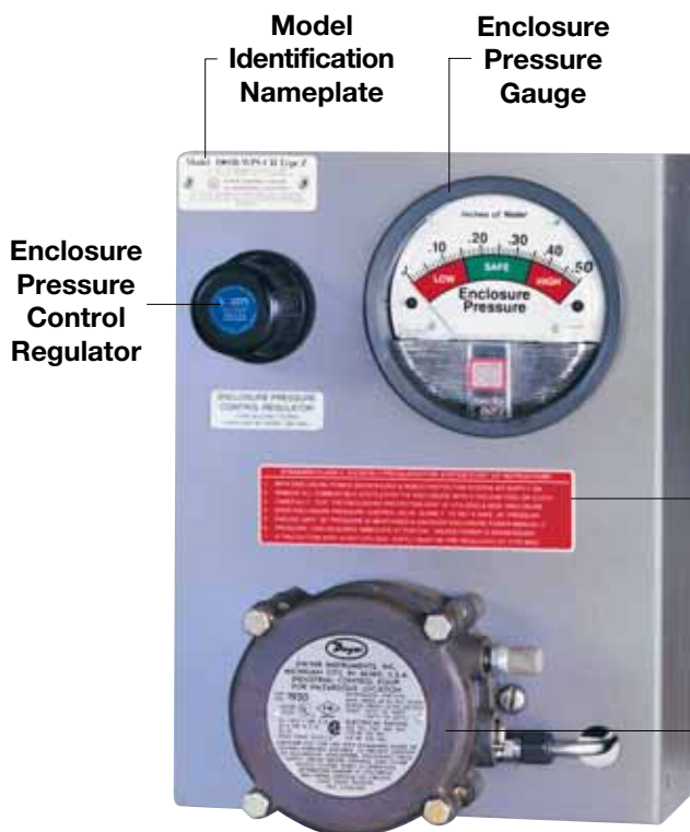
Model 1001B-WPS Front View
