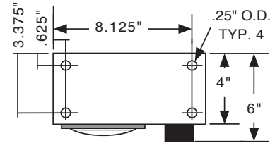
1001B-LPS-BM (Bottom Mount Configuration)
