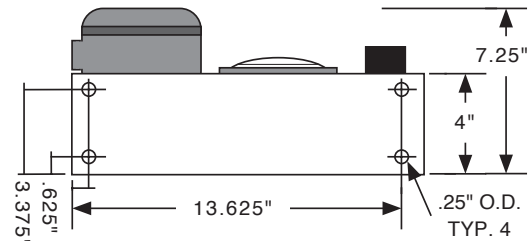
1001B-WPS-TM (Top Mount Configuration)
