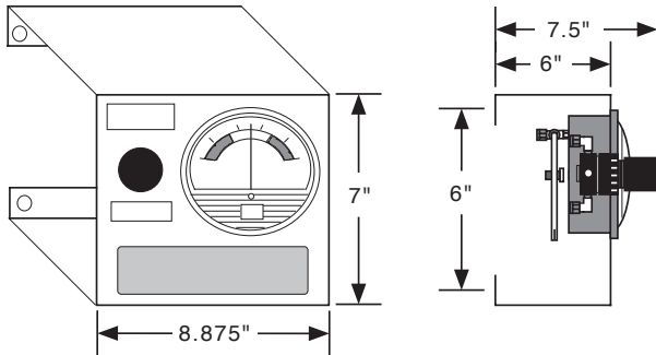
1001B-LPS-WM (Wall Mount Configuration)
