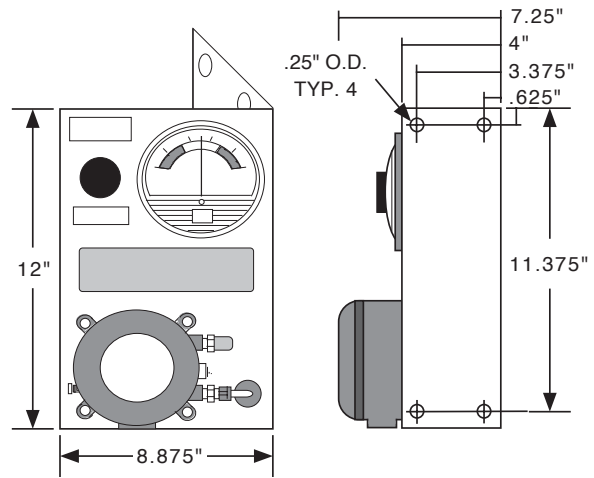
1001B-WPS-LH (Left Hand Configuration)
