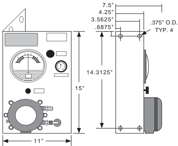
1002-WPS & WPSA-RH (Right Hand Configuration)
