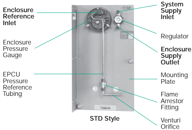
CONNECTION POINTS SHOWN ABOVE IN BOLD TEXT ON SYSTEM DIAGRAM
