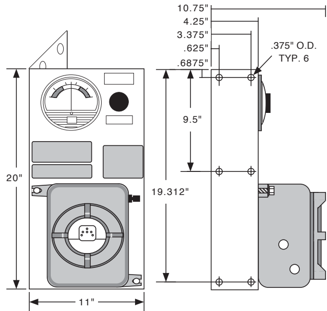
2001B-STD-RH (Right Hand Configuration)
