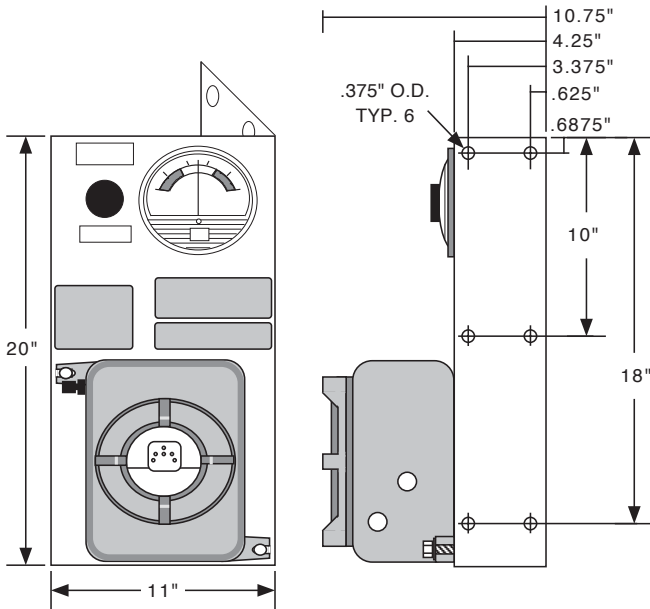
2001B-STD-LH (Left Hand Configuration)
