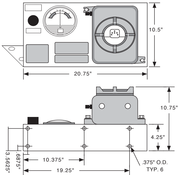
2001B-STD-TM (Top Mount Configuration)
