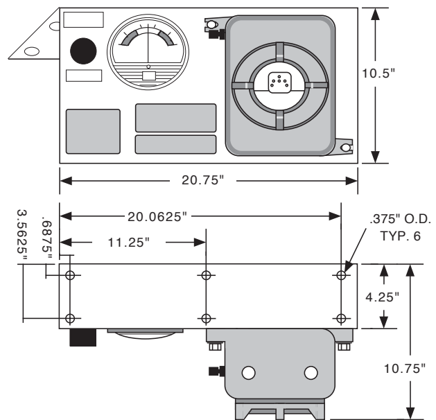
2001B-STD-BM (Bottom Mount Configuration)
