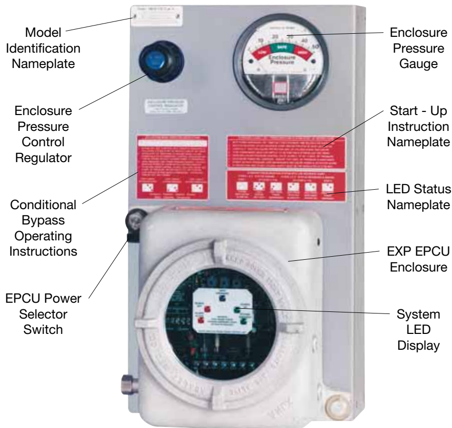
Model 2001B-STD-LH Front View
