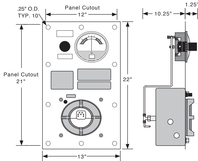
2001B-STD-FM & 2001B-STD-PM (Frame & Panel Mount Configuration)
