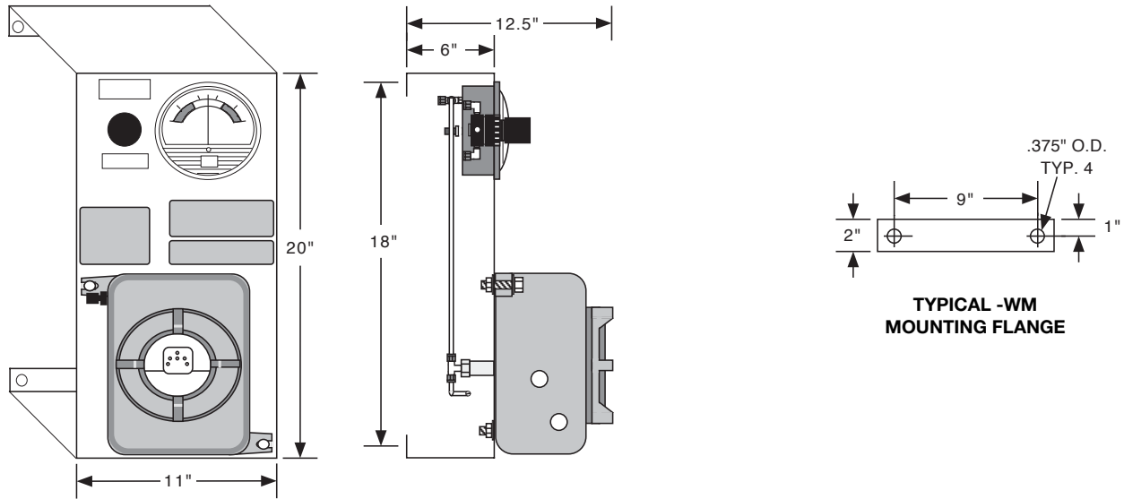
2001B-STD-WM (Wall Mount Configuration)
