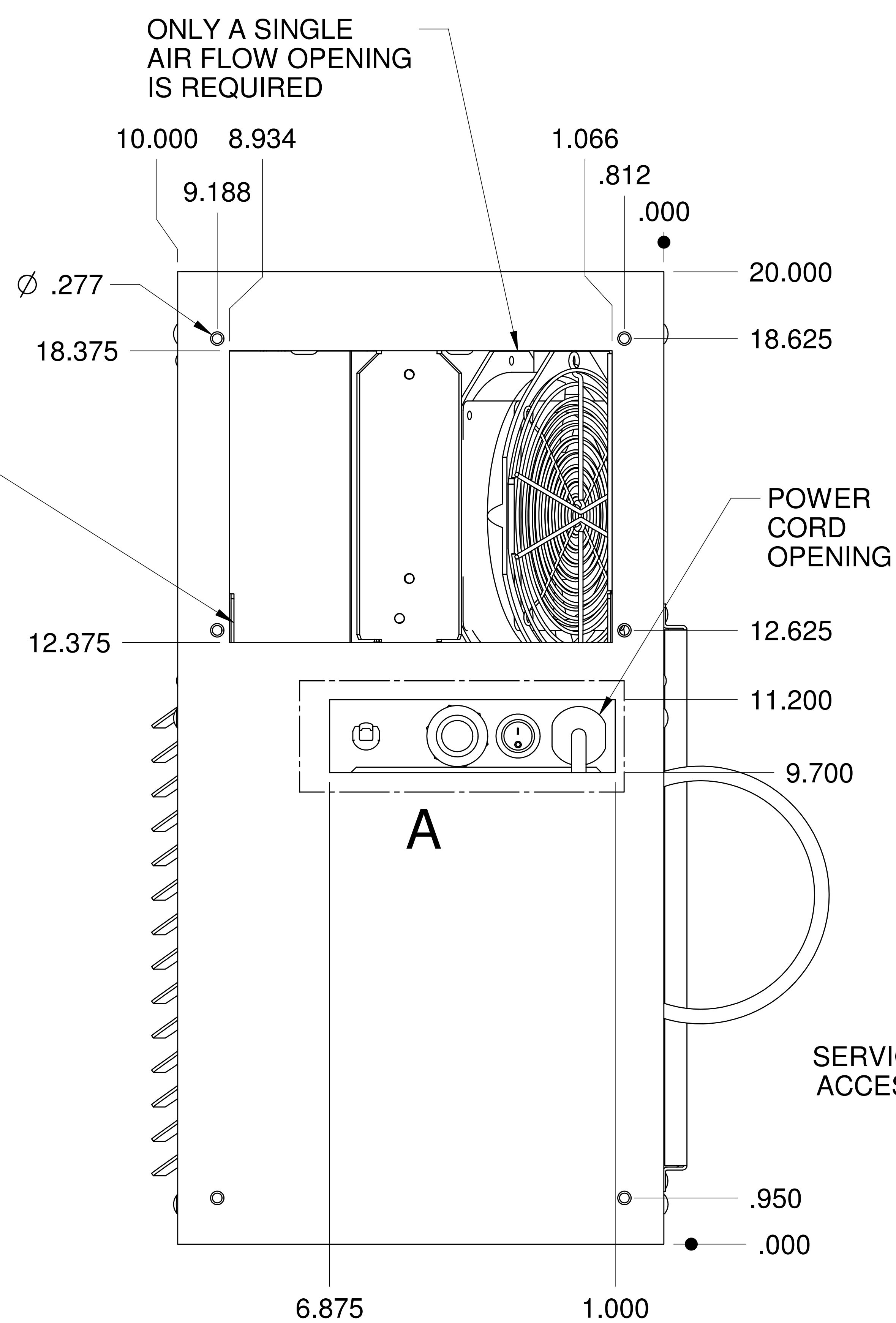
CUTOUT DIMENSIONS AS VIEWED FROM INSIDE ENCLOSURE
