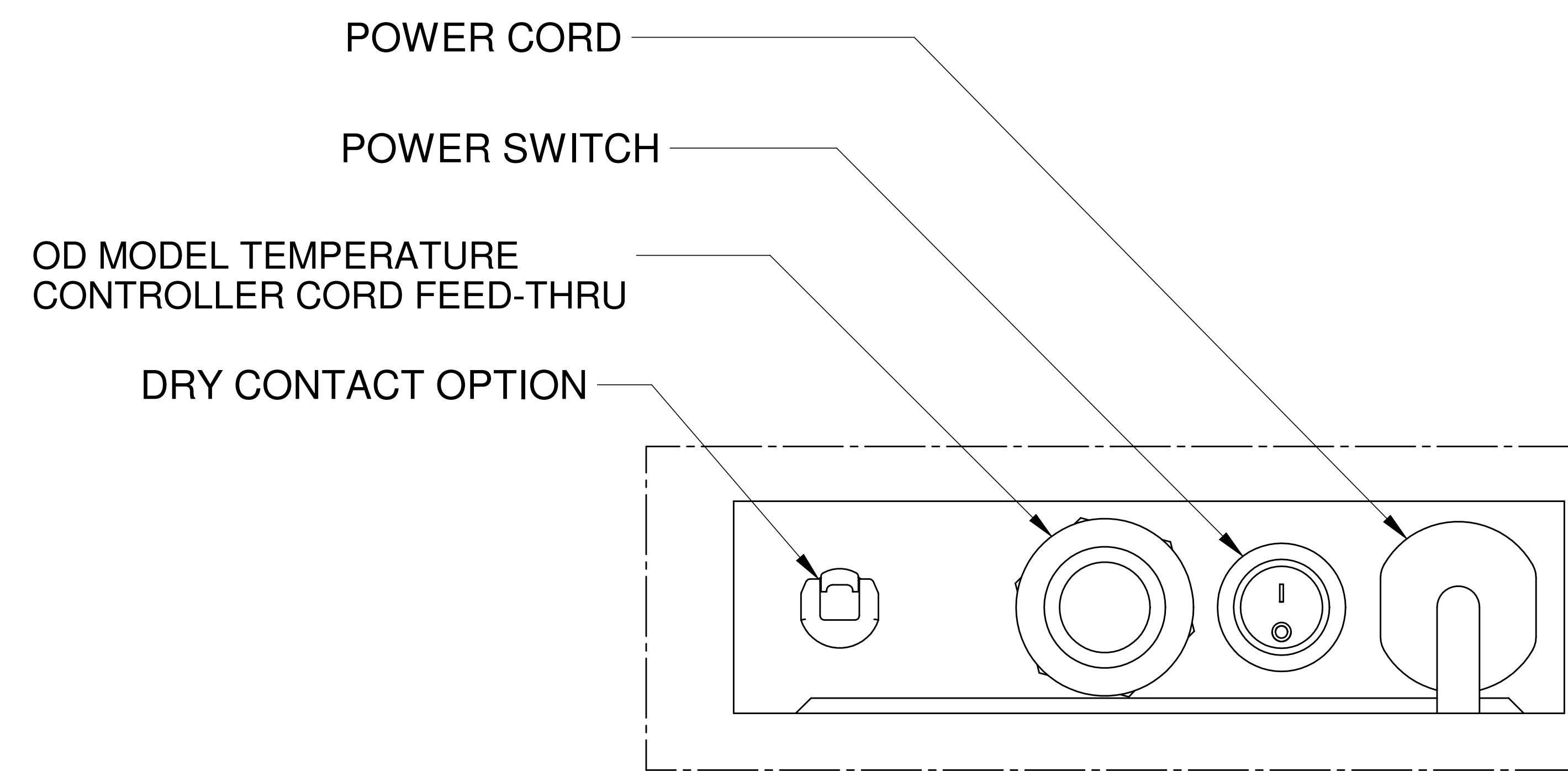
DETAIL A
