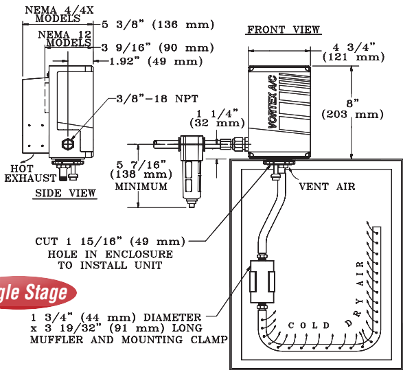
(VORTEX A/C SHOWN TOP MOUNTED ON CUSTOMER'S ENCLOSURE) 900, 1500 AND 2500 BTUH MODELS SHOWN HERE
