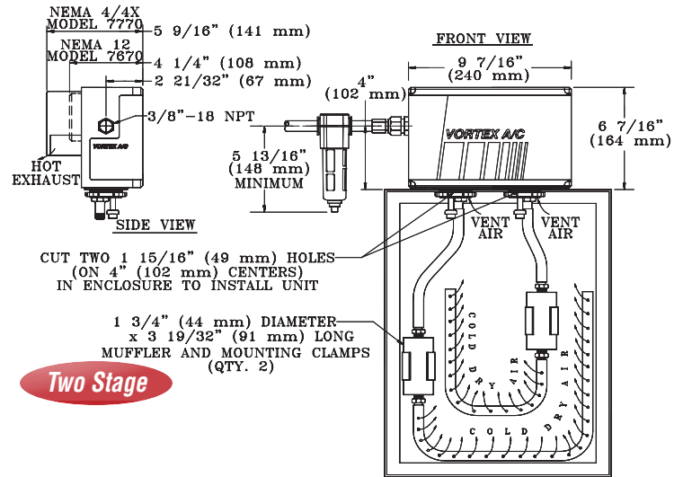
(TWO-STAGE 5000 BTUH VORTEX A/C SHOWN TOP MOUNTED ON CUSTOMER'S ENCLOSURE)
